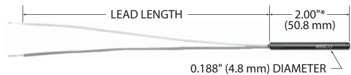
MODEL S482PW IS 2.4\" (60.3 mm) LONG
