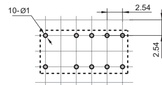
2 coils latching
