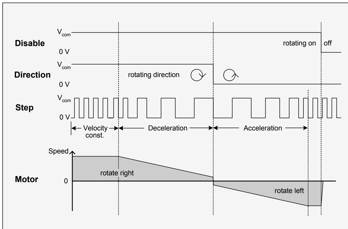
Figure 6.3: Step-Direction signals and motor reactions
