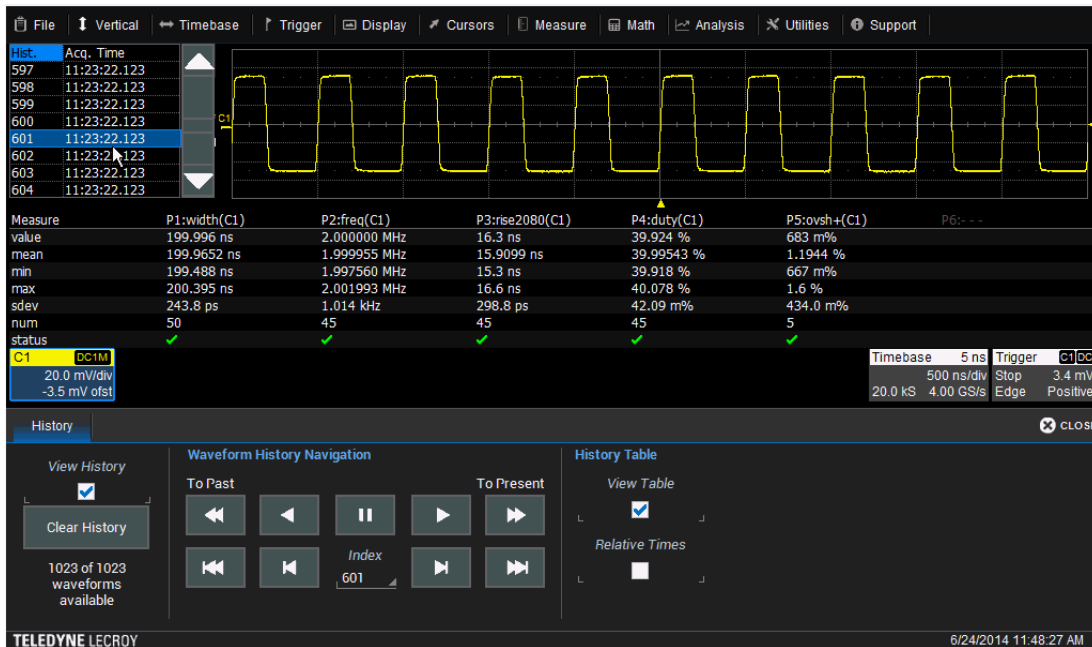
Figure 4: Perform measurement and/or math operations on any acquired waveform in History Mode. In this example, one of a group of single-shot acquisitions is measured for width, frequency, rise time (20-80%), duty cycle, and overshoot.
