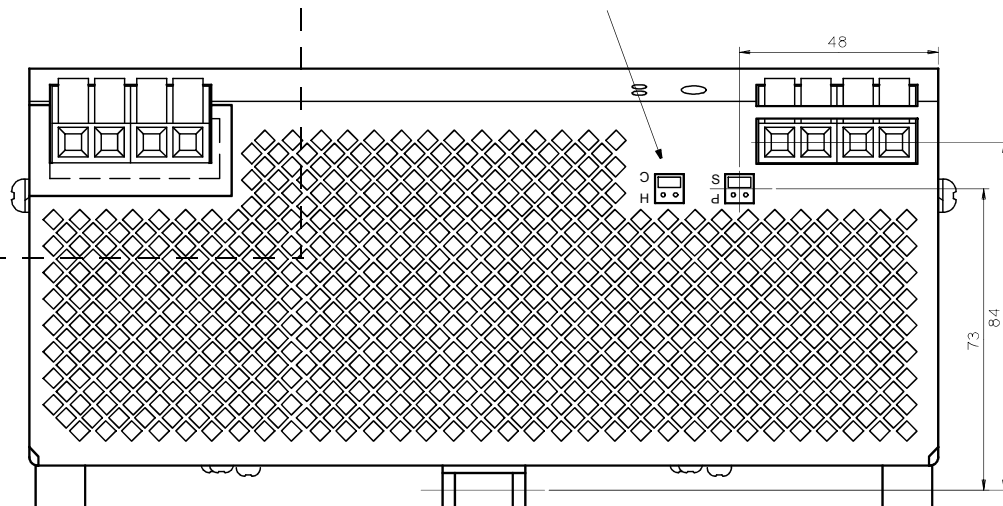
Bottom view SL20
