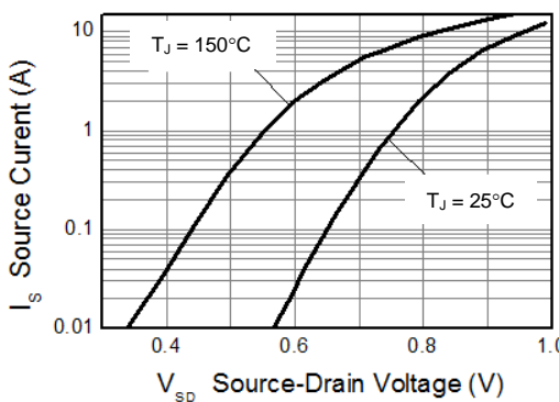
Reverse Diode Characteristic
