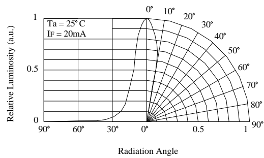
Directivity (Angle : 20^\circ )
