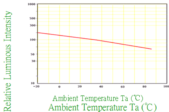
Fig.4 Relative Luminous Intensity-Ta
