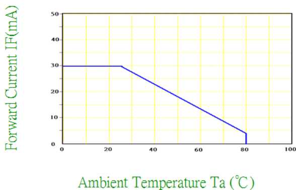
Fig.5 IF-Ta
