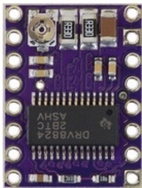
DRV8824 stepper motor driver carrier.
