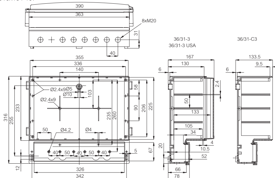
CARDMASTER 383x316x134-167
