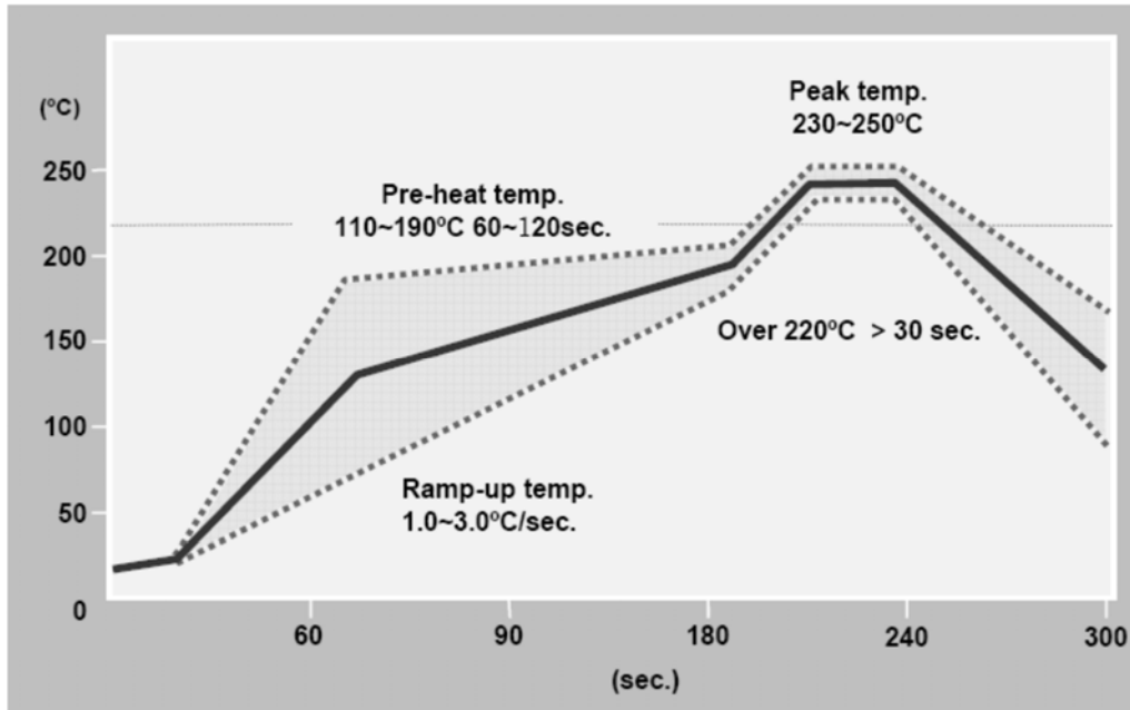
FIGURE 13 – RECOMMENDED SOLDERING PROFILE
