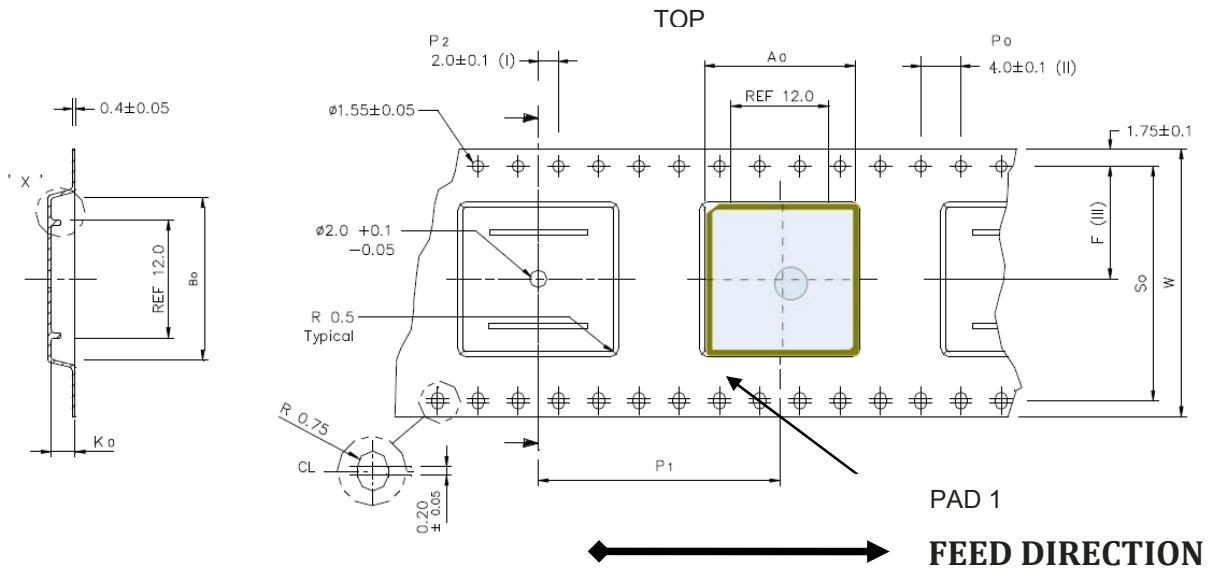
FIGURE 9 – CARRIER
