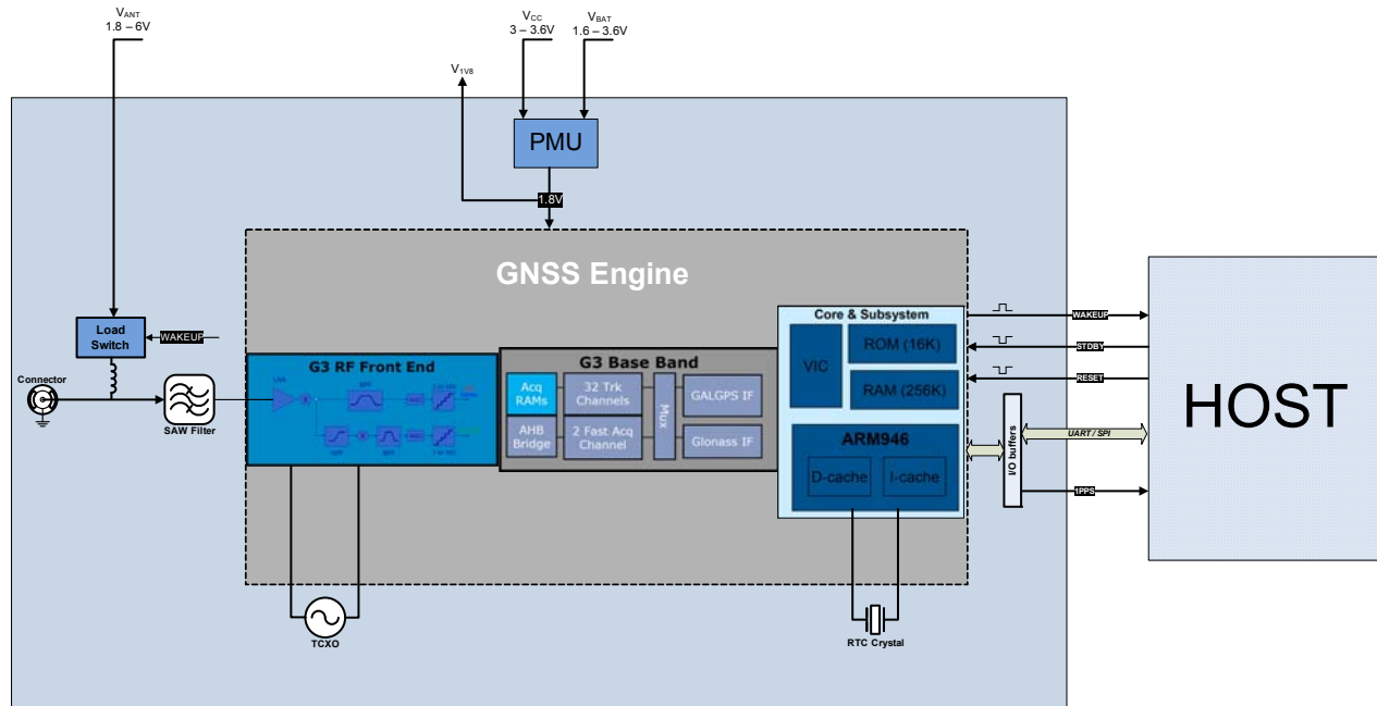
FIGURE 2 – ORG1208 ARCHITECTURE
