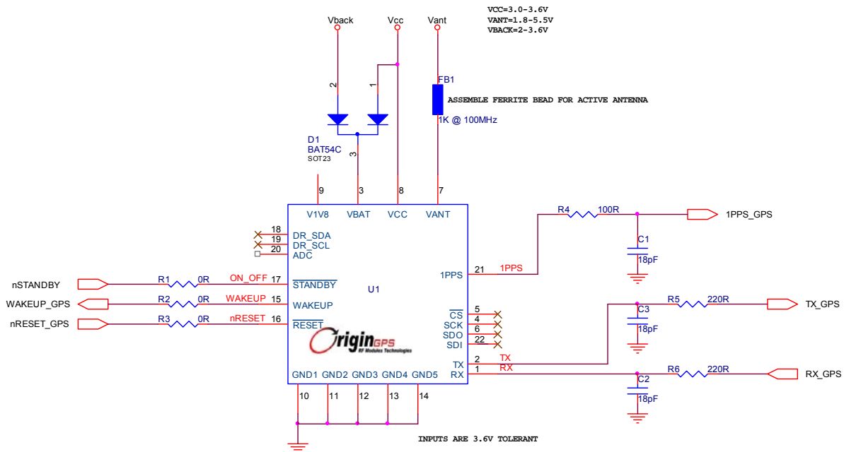
FIGURE 7 – ORG1208 UART INTERFACE CIRCUIT
