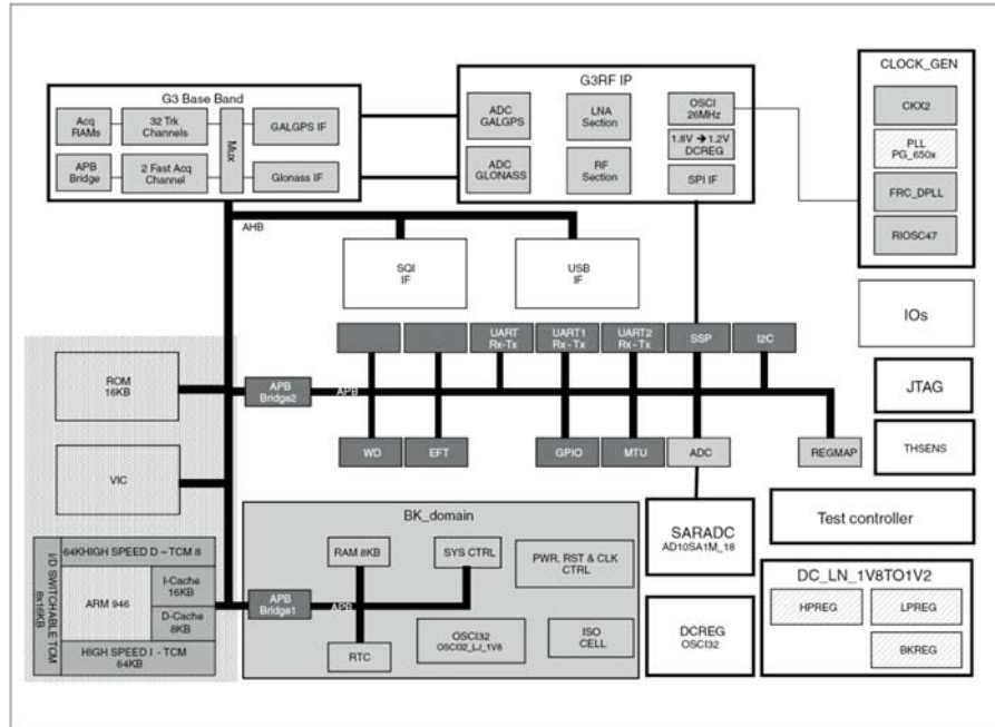
FIGURE 3 – GNSS SoC FUNCTIONAL BLOCK DIAGRAM
