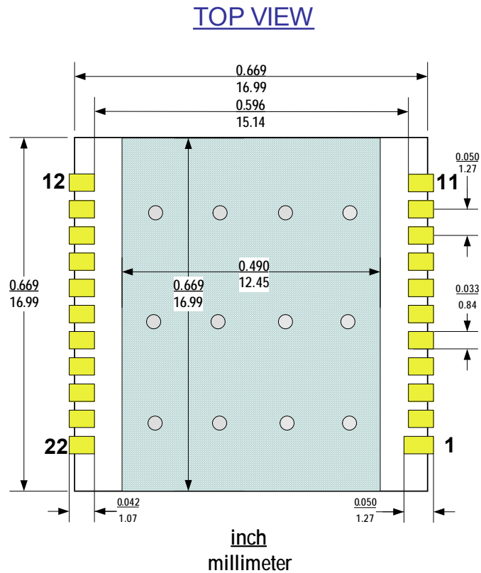
FIGURE 8 – FOOTPRINT
