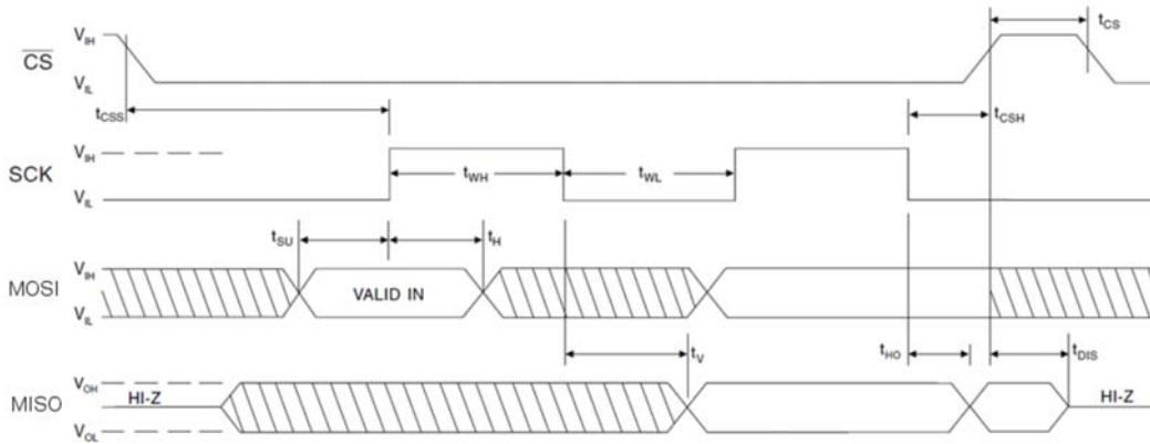
FIGURE 5 – SPI TIMING
