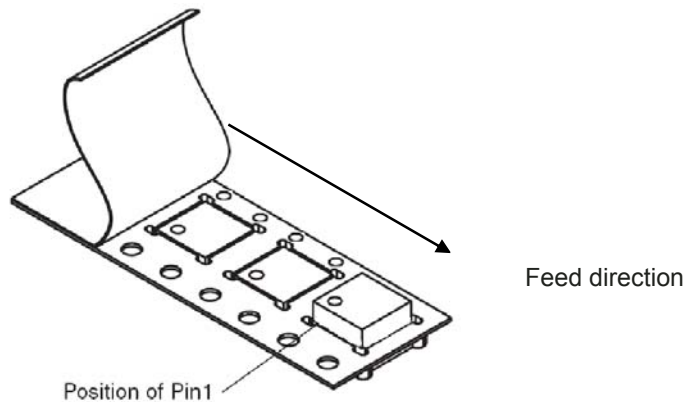
FIGURE 11 – MODULE POSITION
