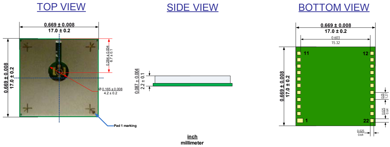
FIGURE 15 – ORG1208 MECHANICAL DRAWING
