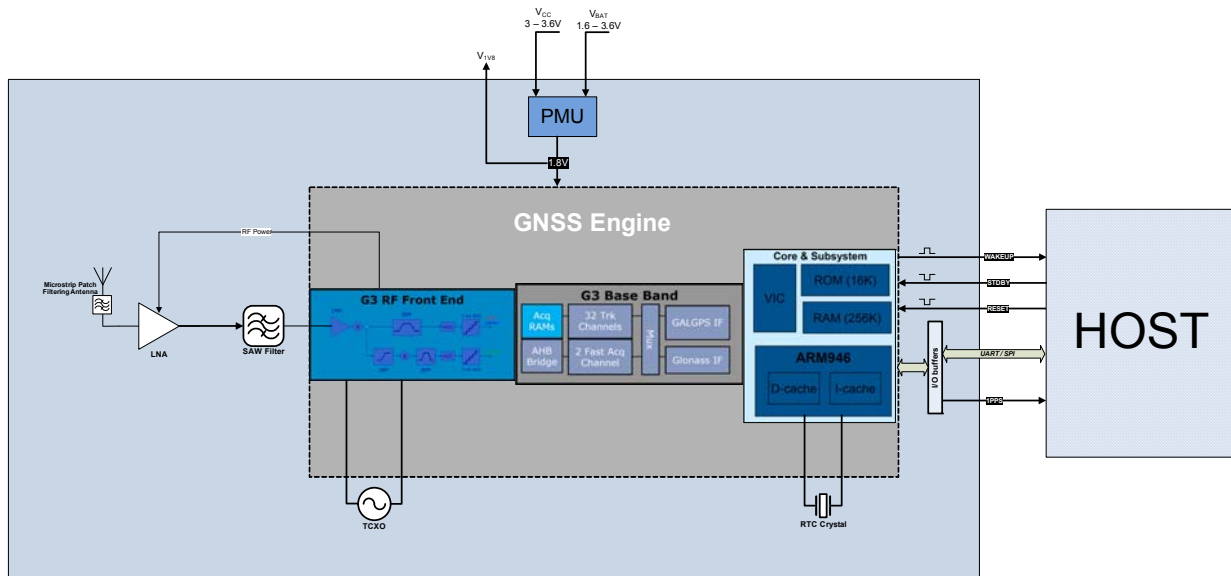
FIGURE 1 – ORG1218 ARCHITECTURE
