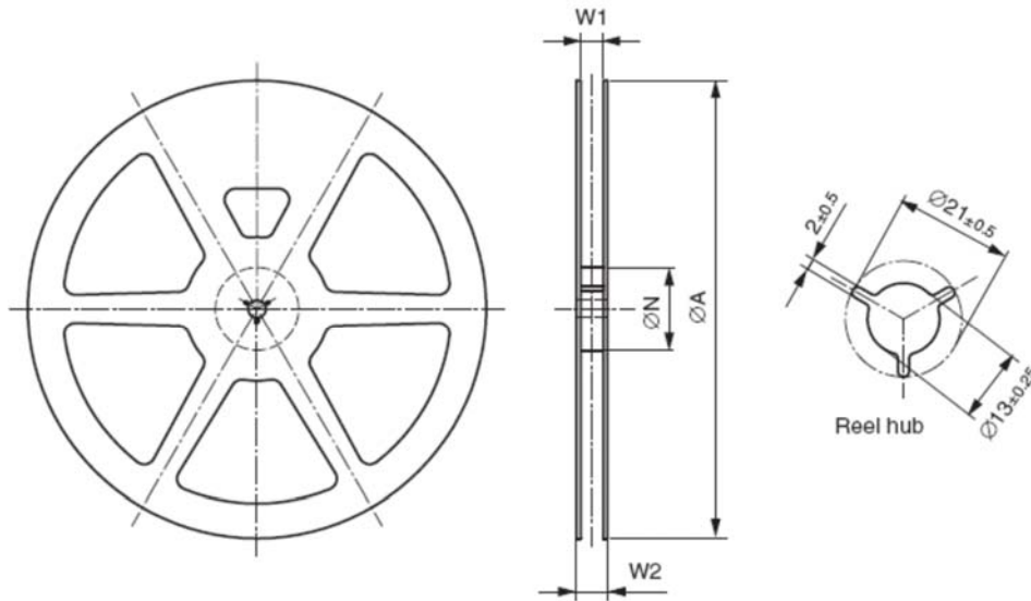
FIGURE 12 – REEL
