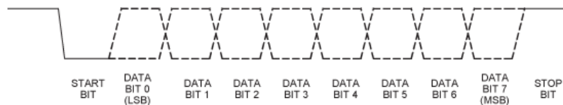
FIGURE 4 – UART INTEGRITY
