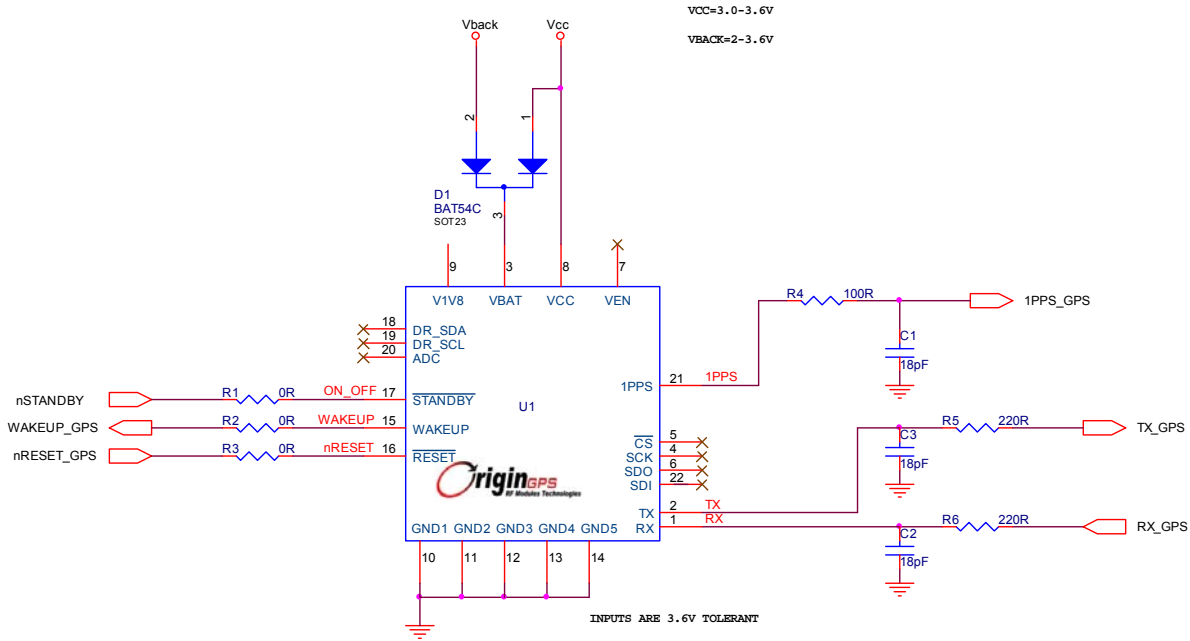
FIGURE 6 – ORG1218 UART INTERFACE CIRCUIT
