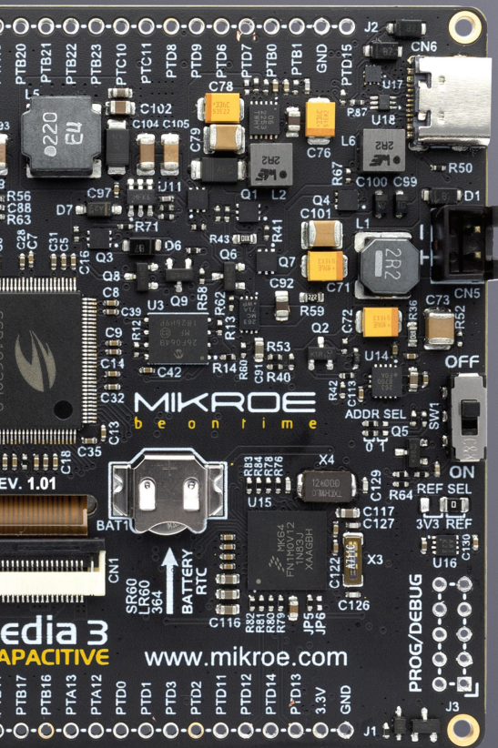
Figure 13: mikromedia 3 back view
