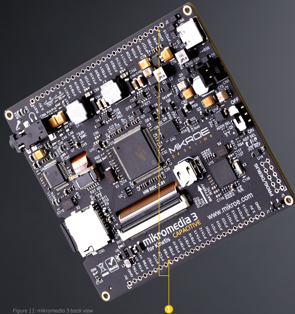
Figure 11: mikromedia 3 back view
