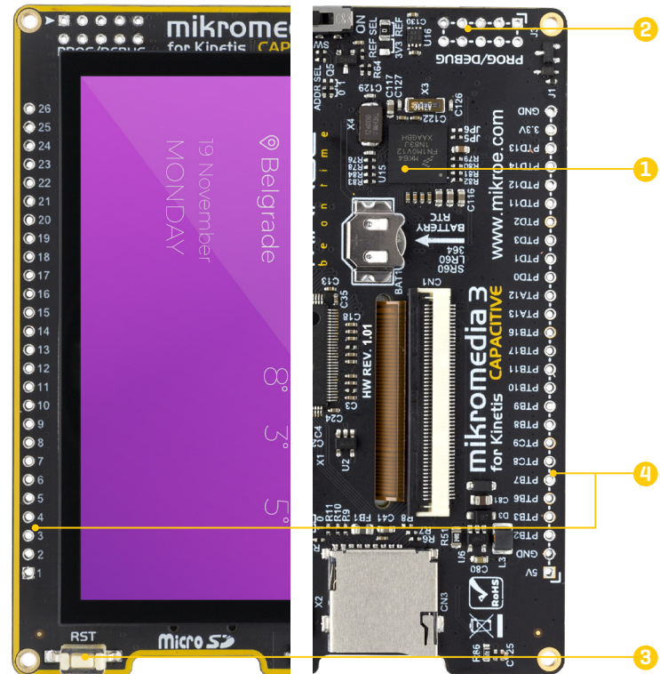
Figure 2: Front and back partial view
