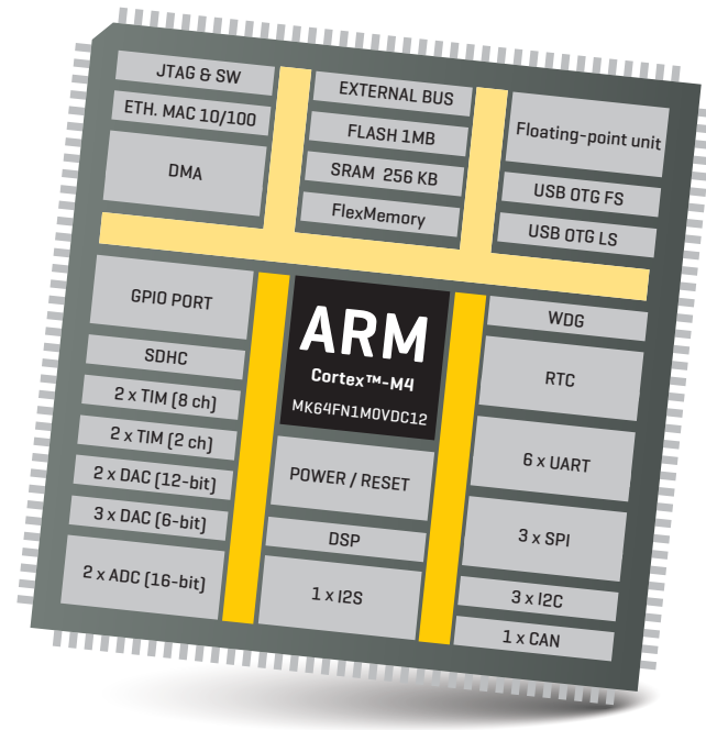
Figure 1: MK64FN1M0VDC12 MCU block schematic
