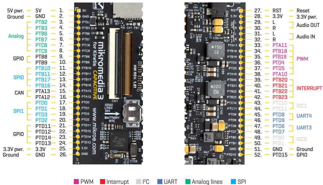
Figure 12: 1x26 pin header view
