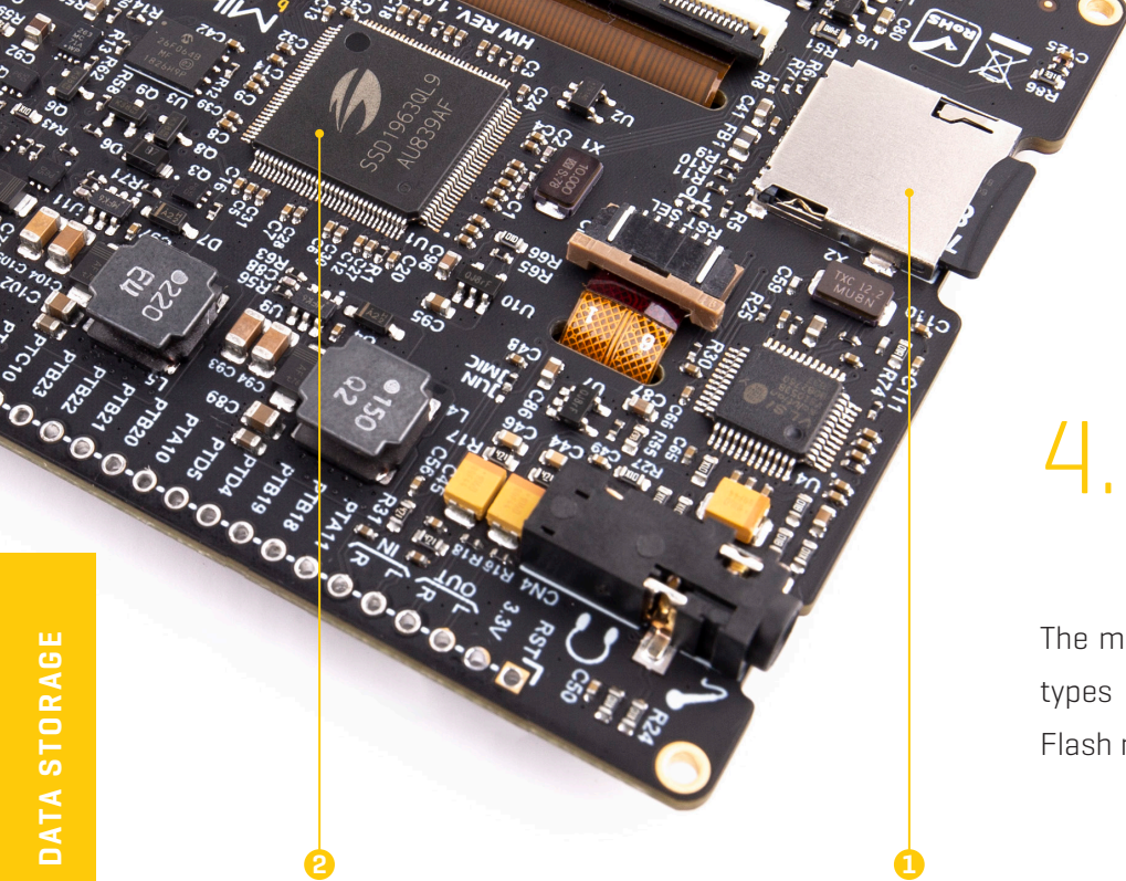
Figure 9: MicroSD card slot view
