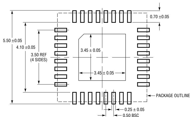
UH Package 32-Lead Plastic QFN (5mm × 5mm) (Reference LTC DWG # 05-08-1693)
