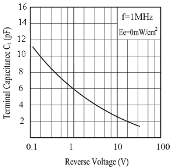
Terminal Capacitance vs. Reverse Voltage
