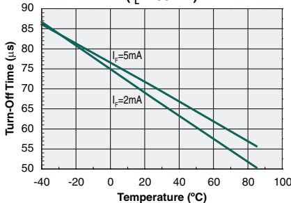
Form-A Typical Turn-Off Time vs. Temperature ( I_L=100\text{mA} )
