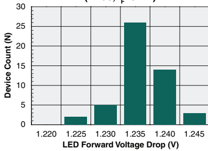
Form-A Typical LED Forward Voltage Drop (N=50, I_F=5\text{mA} )
