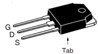
TO-247 (IXTH)
