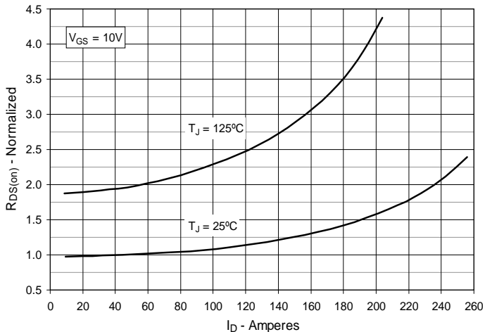
Fig. 5. R_{DS(on)} Normalized to I_D = 37.5\text{A} Value vs. Drain Current
