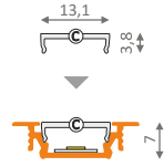
cover click C white transparent
