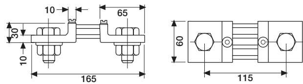
SNT800 ÷ 1000 A/60 mV
