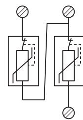
OVR T2 2L 15 75 P
