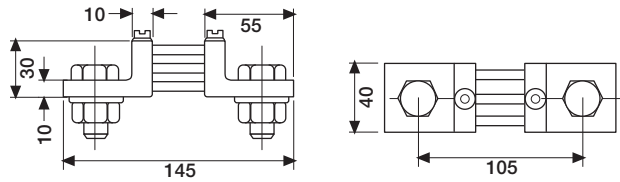
SNT800 ÷ 1000 A/60 mV
