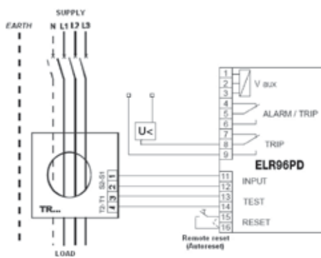
ELR96PD - undervoltage release wiring
