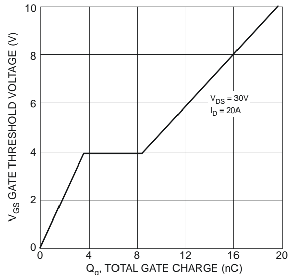
Figure 12 Gate Charge
