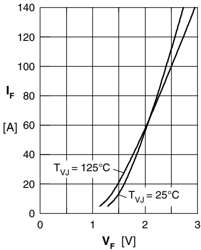
Fig. 1 Typ. ward current I_F versus V_F
