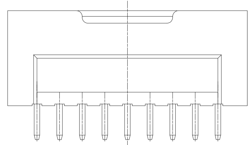
ENGAGEMENT FIGURE (2:1)
