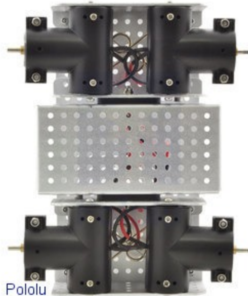
Bottom view of Daggu Wild Thumper 4WD chassis (silver version).
