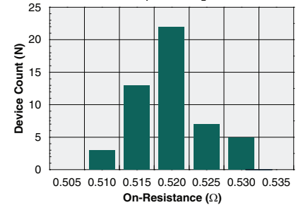
Typical On-Resistance Distribution (N=50, I F =1mA, I L =0.6A)
