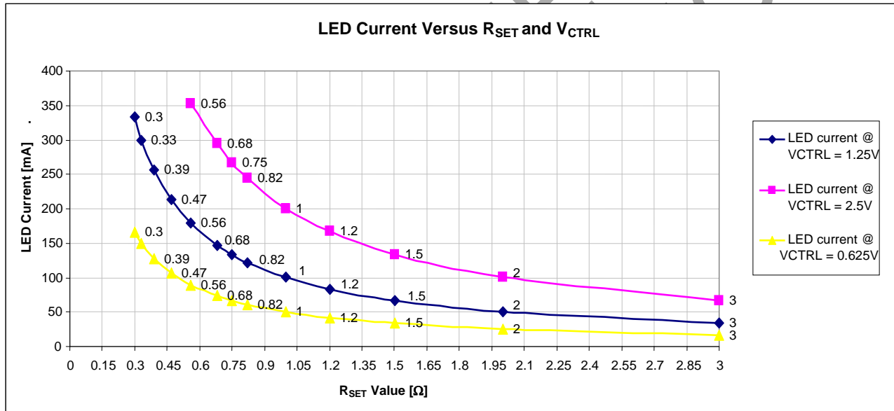
Figure 4 LED Current Setting vs. R SET and V CTRL
