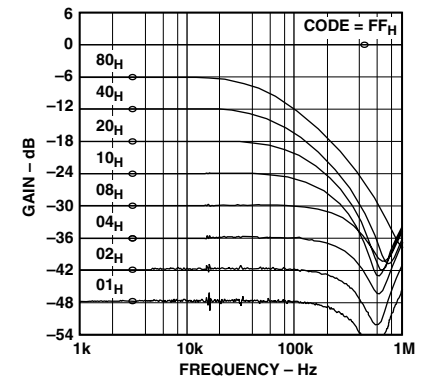
TPC 18. 100 k \Omega Gain vs. Frequency vs. Code
