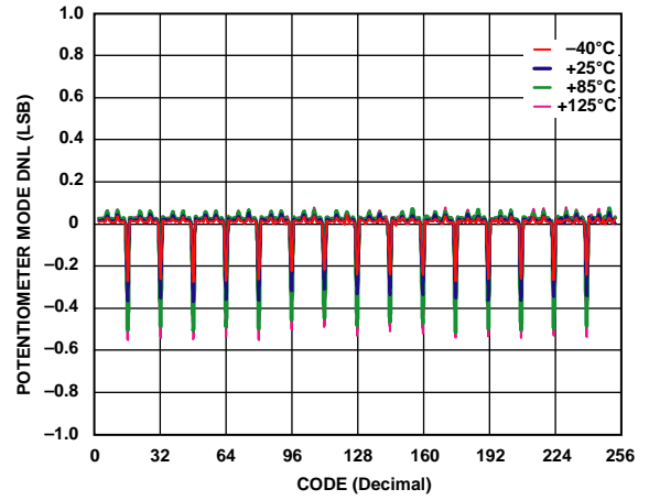
Figure 7. DNL vs. Code, V_{DD} = 5 V
