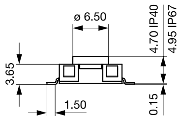
SMS Gullwing Base module
