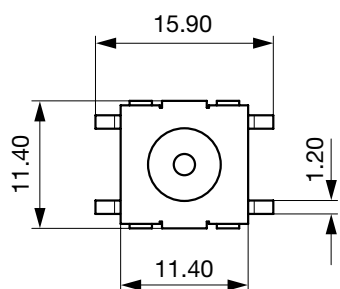
SMS Gullwing Variable height
