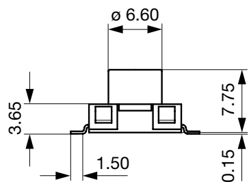
SMS Gullwing Variable height
