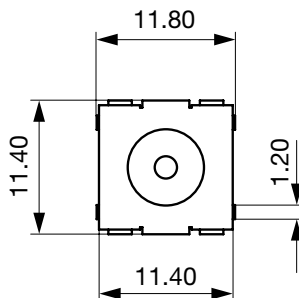
SMS J-lead Variable height
