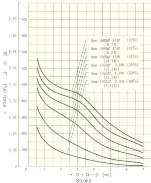
(N) gf Stroke and Pull Force Characteristics
