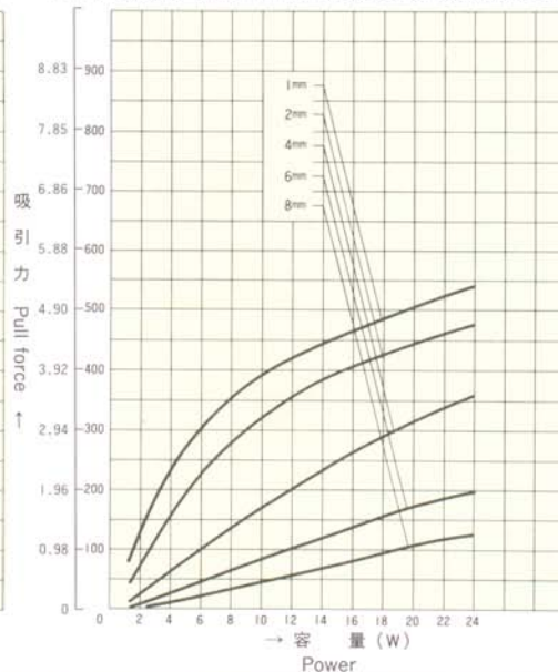
(N) gf Power and Pull Force Characteristics
