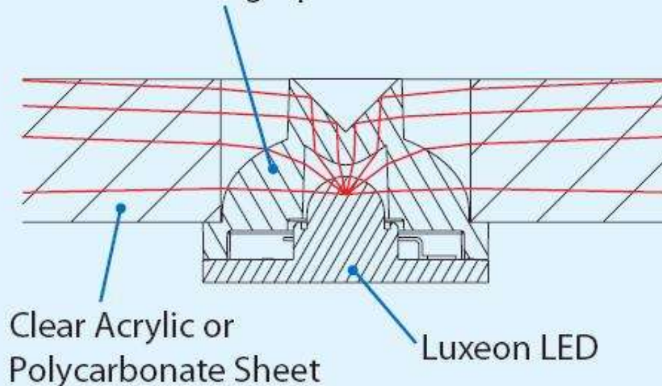
Side-Emitting Optic
