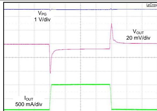
Figure 30. Load Transient Response ( V_{OUT} = 5.0\text{ V} ) V_{IN} = 5.5\text{ V} , I_{OUT} = 100\text{ mA} to 1\text{ A} to 100\text{ mA} at 1\text{ A}/\mu\text{s} , C_{OUT} = 10\ \mu\text{F} , V_{PG} = V_{OUT}
