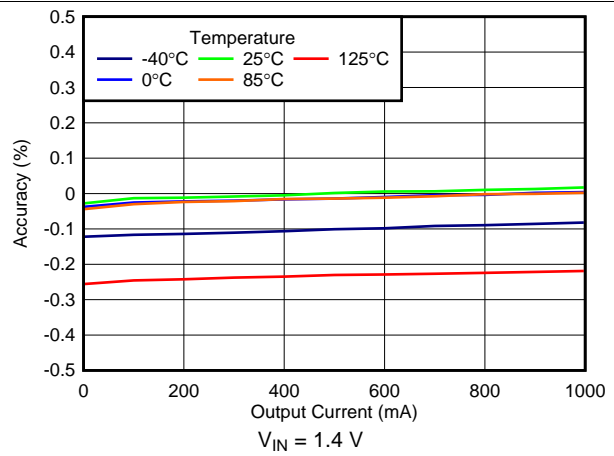
Figure 16. Load Regulation
