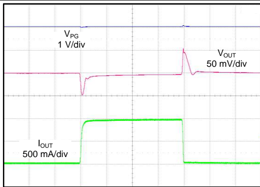
Figure 29. Load Transient Response ( V_{OUT} = 1.2\text{ V} ) V_{IN} = 1.5\text{ V} , I_{OUT} = 100\text{ mA} to 1\text{ A} to 100\text{ mA} at 1\text{ A}/\mu\text{s} , C_{OUT} = 10\ \mu\text{F} , V_{PG} = V_{OUT}
