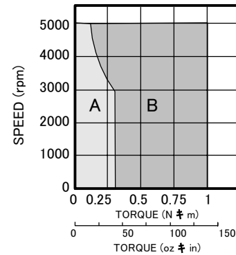
SGMAH-01B
