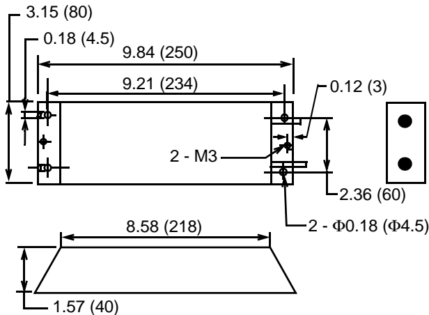
Part#RH500N25_OHMK
