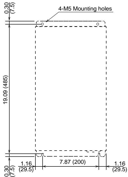
Mounting Hole Diagram
