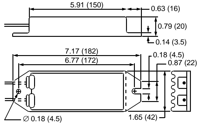
Part#RH120 50 OHMJ
