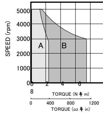
SGMAH08A
