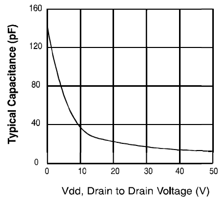
Figure 8. Typical Output Capacitance
