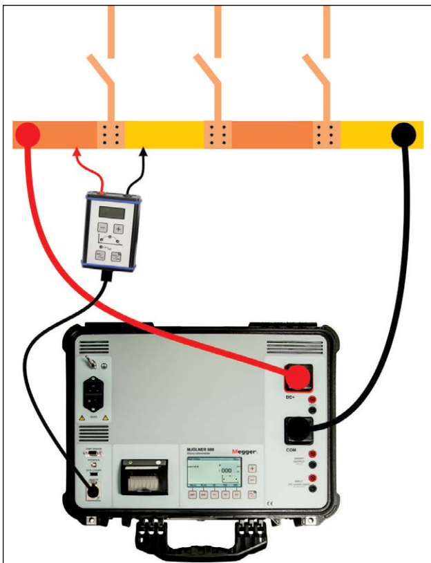
Using the remote control you can measure the voltage drop (voltage) across each contact element within every section of the bus-bar being tested.
