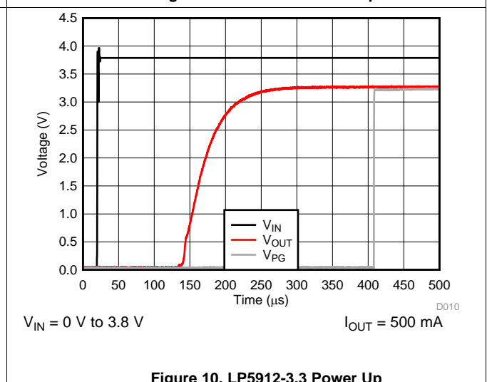
Figure 10. LP5912-3.3 Power Up
