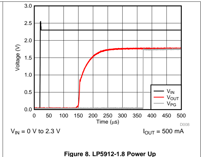
Figure 8. LP5912-1.8 Power Up
