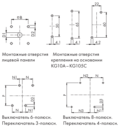
VE KG10A – KG105C + VE1 KG125 – KG162
