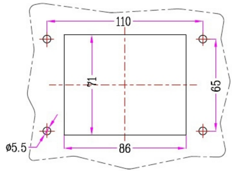
Bulkhead mounting Panel cut out
