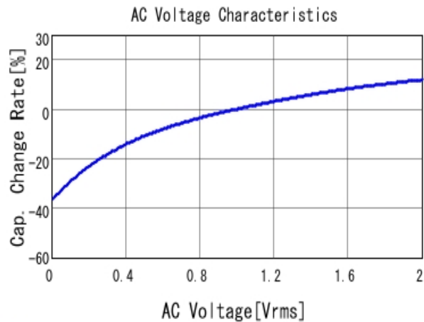
■ GRM188R71C105KE15 C-AC Voltage capchange, DCOV, 25.0d
