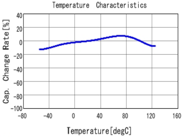
■ GRM188R71C105KE15 C-Temp. capchange, DCO. 0V, ACO. 5Vrm
