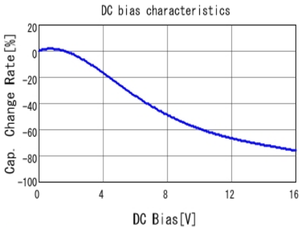
■ GRM188R71C105KE15 C-DC bias capchange, 25.0degC, AC1V
