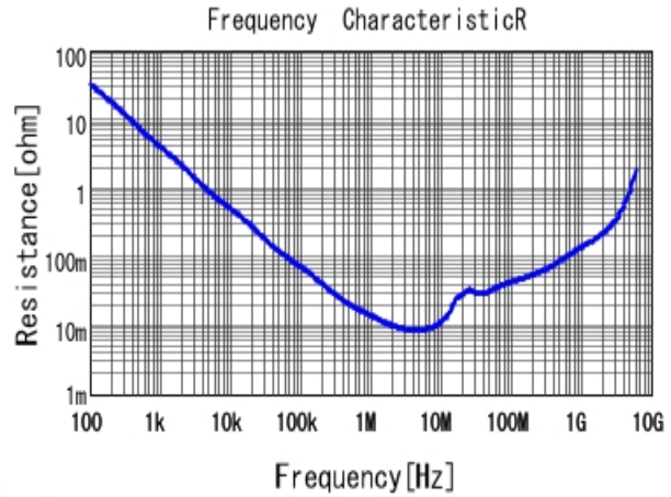
■ GRM188R71C105KE15 R DCOV, 25degC
