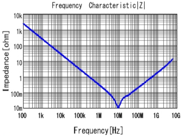
■ GRM188R71C105KE15 |Z| DCOV, 25degC
