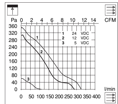
D341Q, 343Q, 344Q, 351Q 12 V DC
