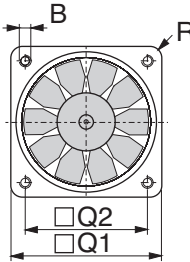
D341T, 343T, 344T, 351T 24 V DC
