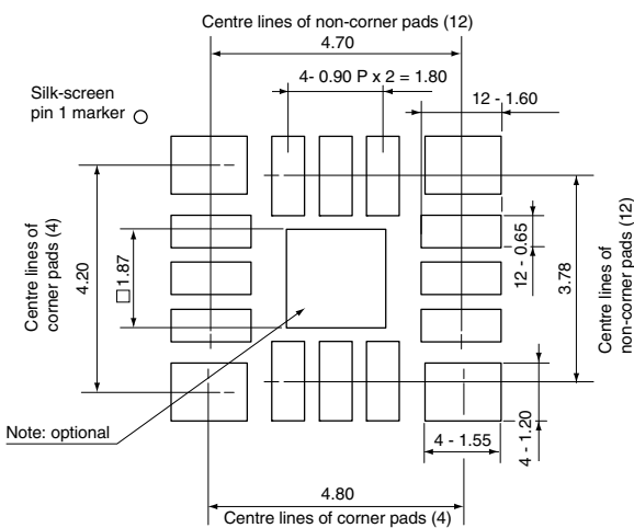
Figure 7.2 Recommended Pad Layout (CRM100)
