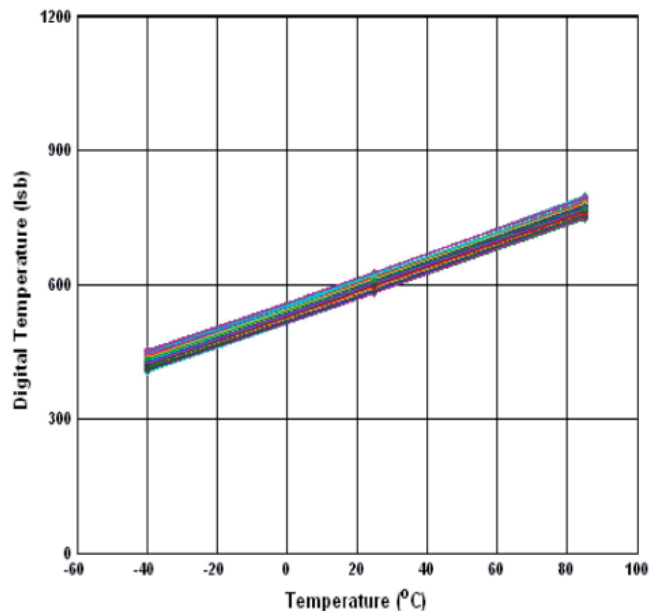
Figure 5.30 Digital Temperature vs Temperature
