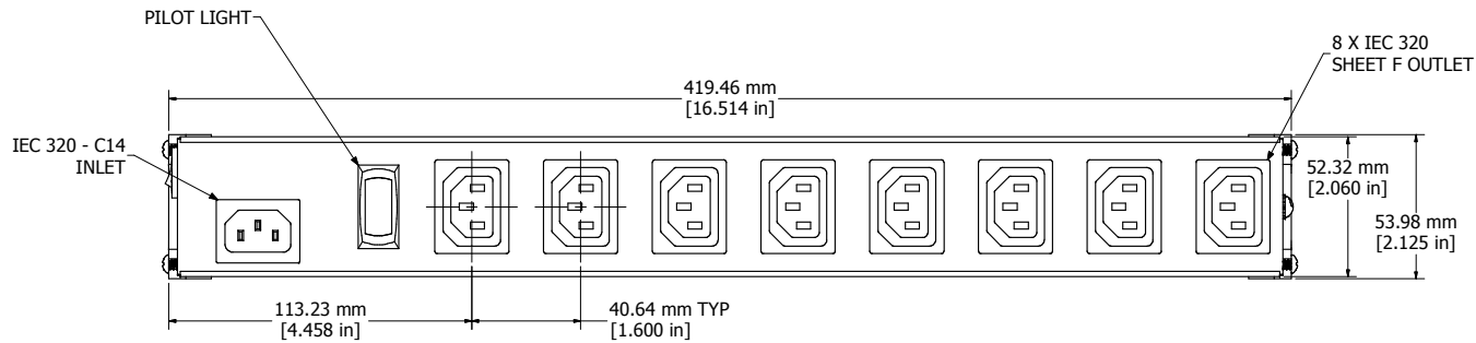
ASSEMBLY - VIEW FROM TOP
