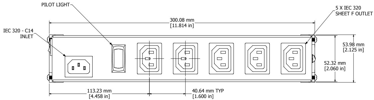
ASSEMBLY - VIEW FROM TOP
