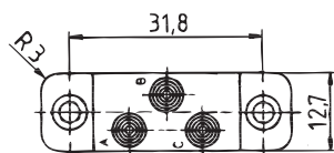
Dimensional drawing of socket terminal strip
