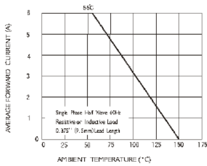
FIG.1-MAXIMUM AVERAGE FORWARD CURRENT DERATING
