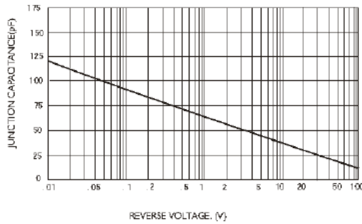
FIG.5-TYPICAL JUNCTION CAPACITANCE
