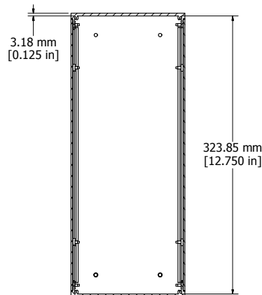
SECTION TT-TT
