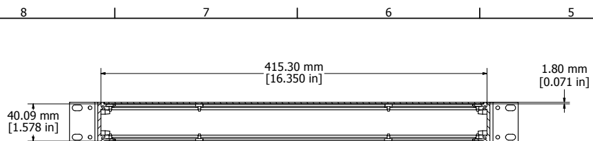
SECTION KK-KK
