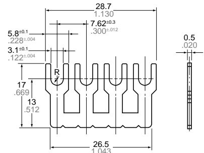
General tolerance \pm 0.5 \pm .020
