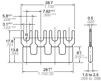
General tolerance \pm 0.5 \pm .020
