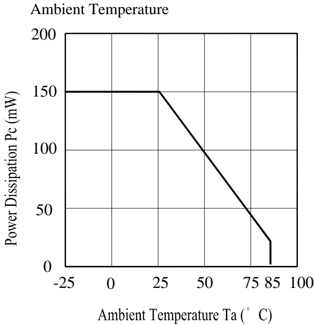
Fig.1 Power Dissipation vs. Ambient Temperature
