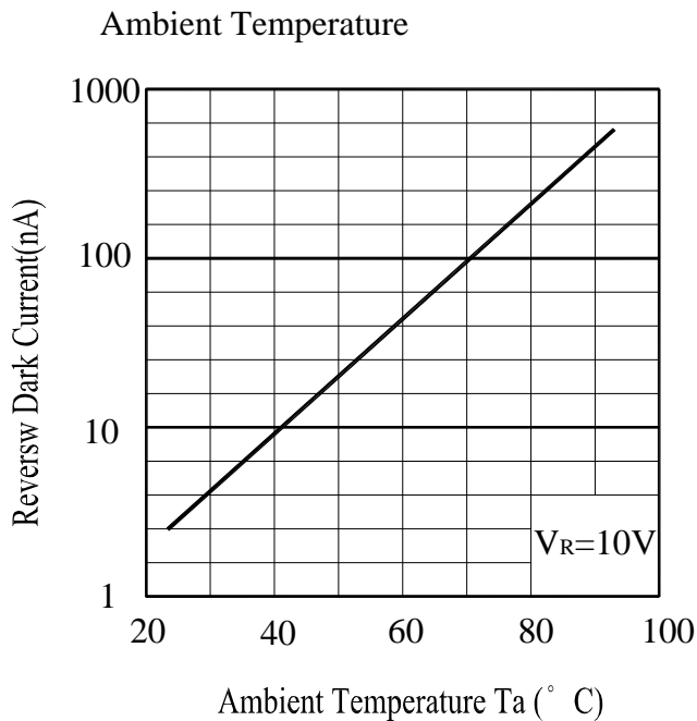
Fig.3 Dark Current vs. Ambient Temperature
