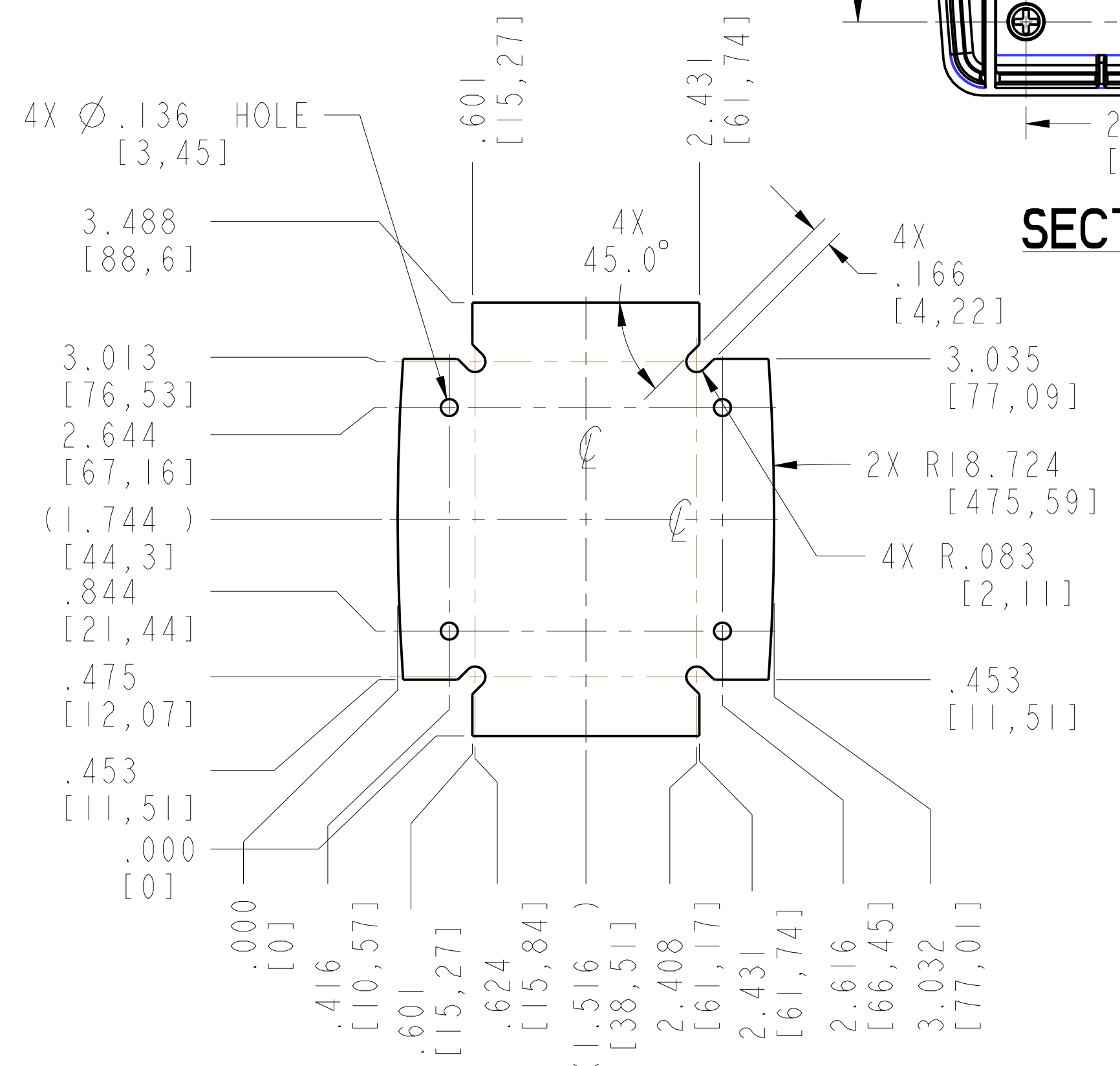
PC BOARD BOTTOM COVER MAX PCB SIZE, .063 TK
