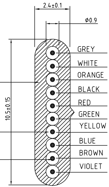
SECTION K-K
